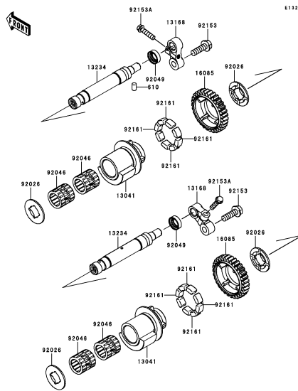
B-12 Balancer
