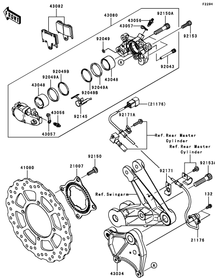
F-12 Rear Brake
