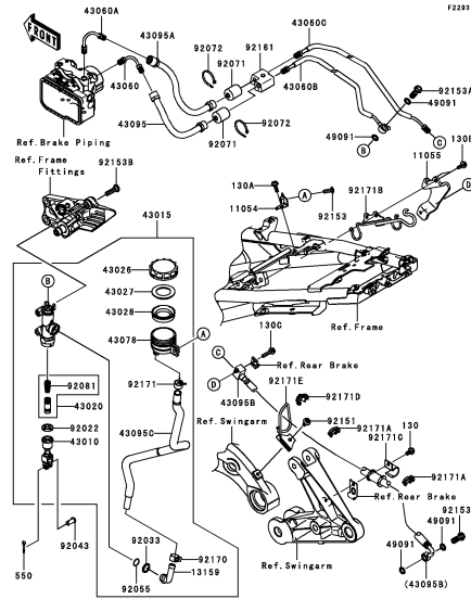
F-10 Rear Master Cylinder(1/2)
