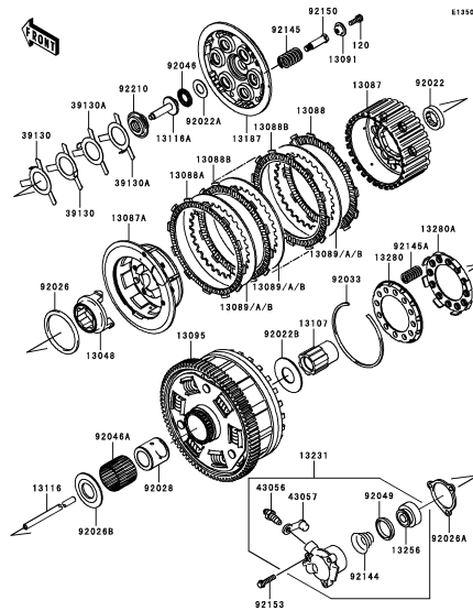
B-13 Clutch(1/2)
