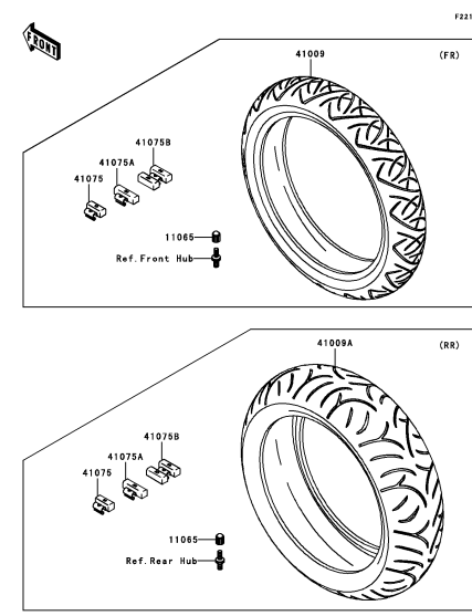
E-14 Tires
