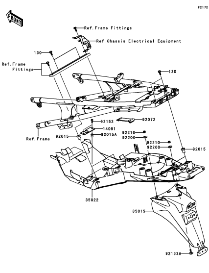
E-12 Rear Fender(s)
