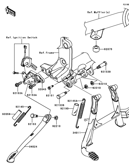
E-13 Stand(s)
