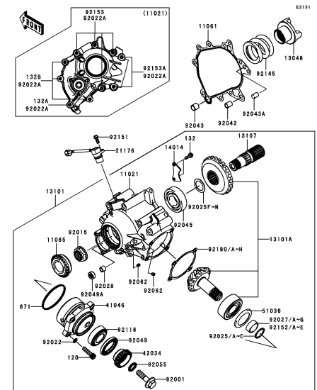
D-8 Front Bevel Gear(1/2)
