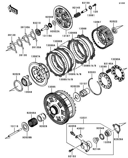
B-14 Clutch(2/2)
