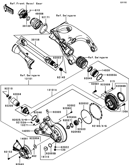
D-10 Drive Shaft/Final Gear(1/2)
