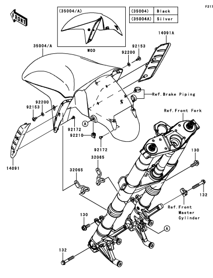
E-11 Front Fender(s)
