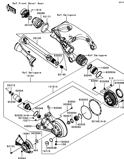
D-11 Drive Shaft/Final Gear(2/2)
