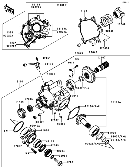
D-9 Front Bevel Gear(2/2)
