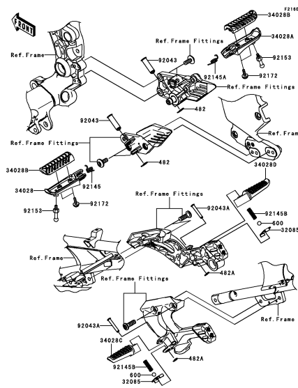
E-10 Footrests
