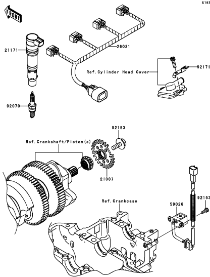
D-3 Ignition System
