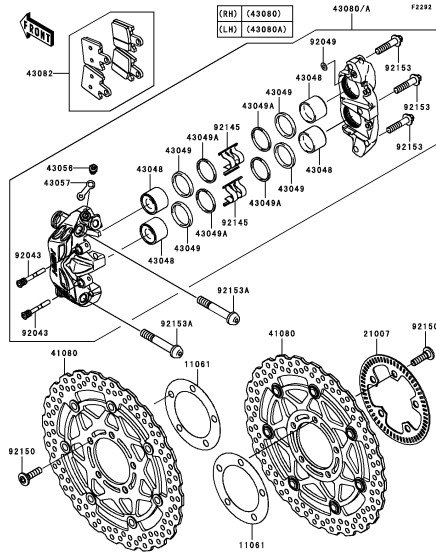
F-9 Front Brake
