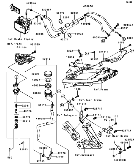
F-11 Rear Master Cylinder(2/2)
