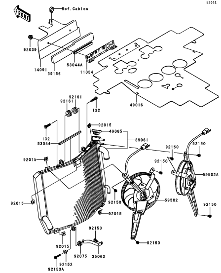
D-5 Radiator
