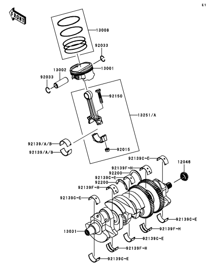
B-11 Crankshaft/Piston(s)
