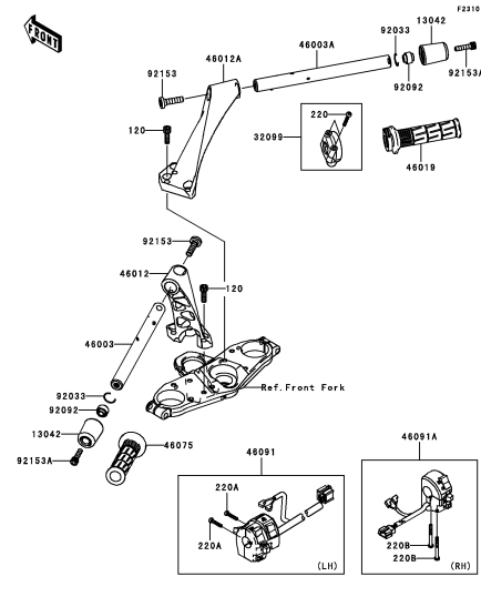
F-13 Handlebar
