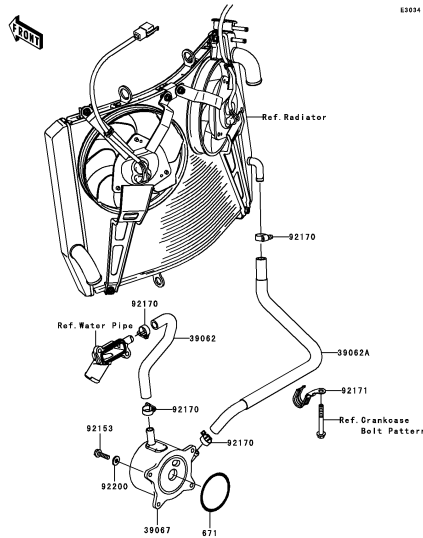
D-6 Oil Cooler
