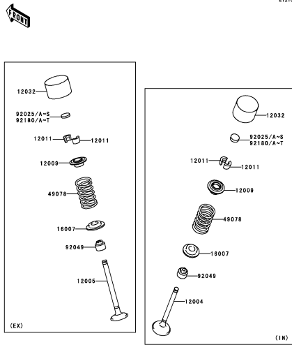
B-9 Valve(s)(2/2)
