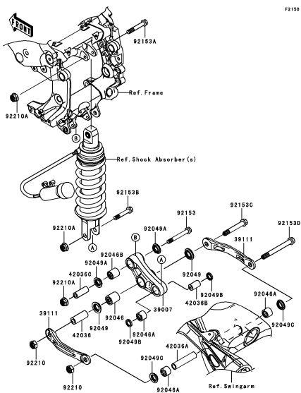
E-9 Suspension
